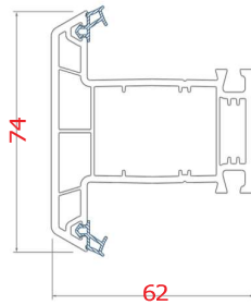
GNC - 621 - T01 T Mullion
