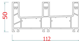
GNS - 620 - F03 3 Track Outer Frame
