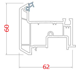
GNC - 621 - T03 Fly Mullion
