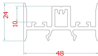
GNS - 620 - A01 Inline Sash Adapter
