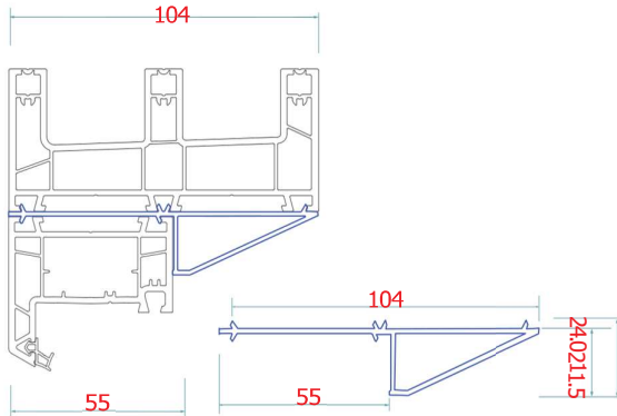
ANA - ALM - A03 104/55 Coupler for 3 Track
