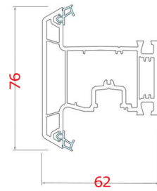
GNC - 621 - S01 Outward Opening Window Sash / T Mullion
