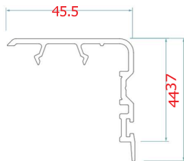
GNS - 620 - L01 Interlock for Window Sash
