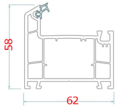
GNC - 621 - F01 Window Outer Frame
