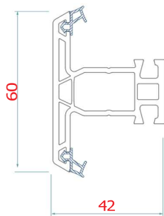
GNS - 621 - T01 T Mullion
