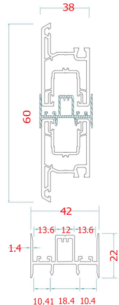
ANA - ALM - A07 In-line Sash Adaptor
