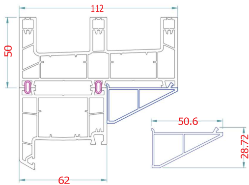
ANA - ALM - A05 112/62 Coupler for 3 Track
