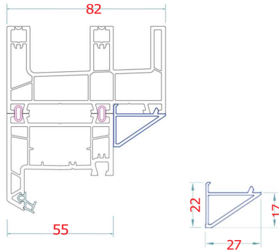
ANA - ALM - A02 82/55 Coupler for 2.5 Track
