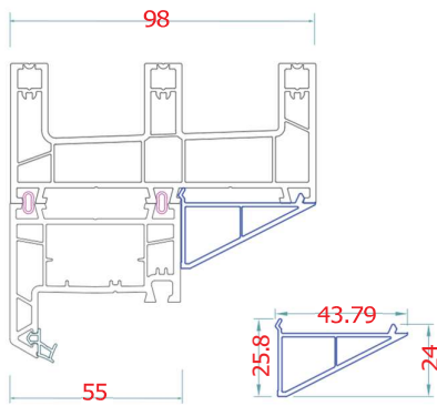
ANA - ALM - A01 98/55 Coupler for 3 Track
