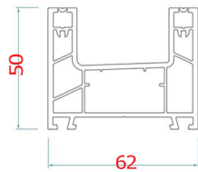
GNS - 620 - F01 2 Track Outer Frame
