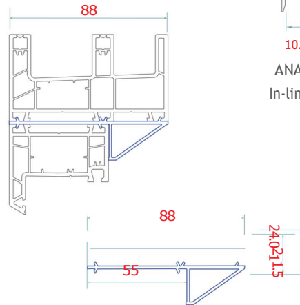
ANA - ALM - A04 88/55 Coupler for 2.5 Track
