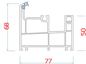
GNS - 621 - F04 Mono Rail Frame
