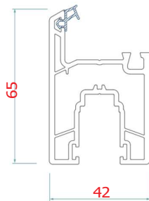
GNS - 621 - S02 Window Super Sash
