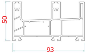
GNS - 620 - F02 2.5 Track Outer Frame
