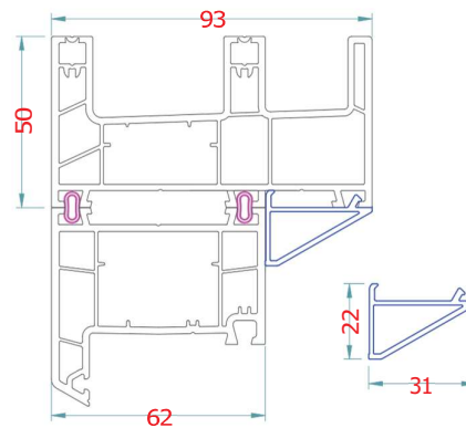
ANA - ALM - A06 93/62 Coupler for 2.5 Track
