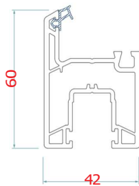
GNS - 621 - S01 Window Sash
